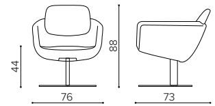
AA 809P base a piastra • plate base
